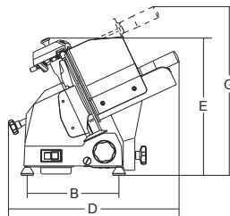
Affilatoio incorporato 195-220 Without built-in sharpener 195-220
